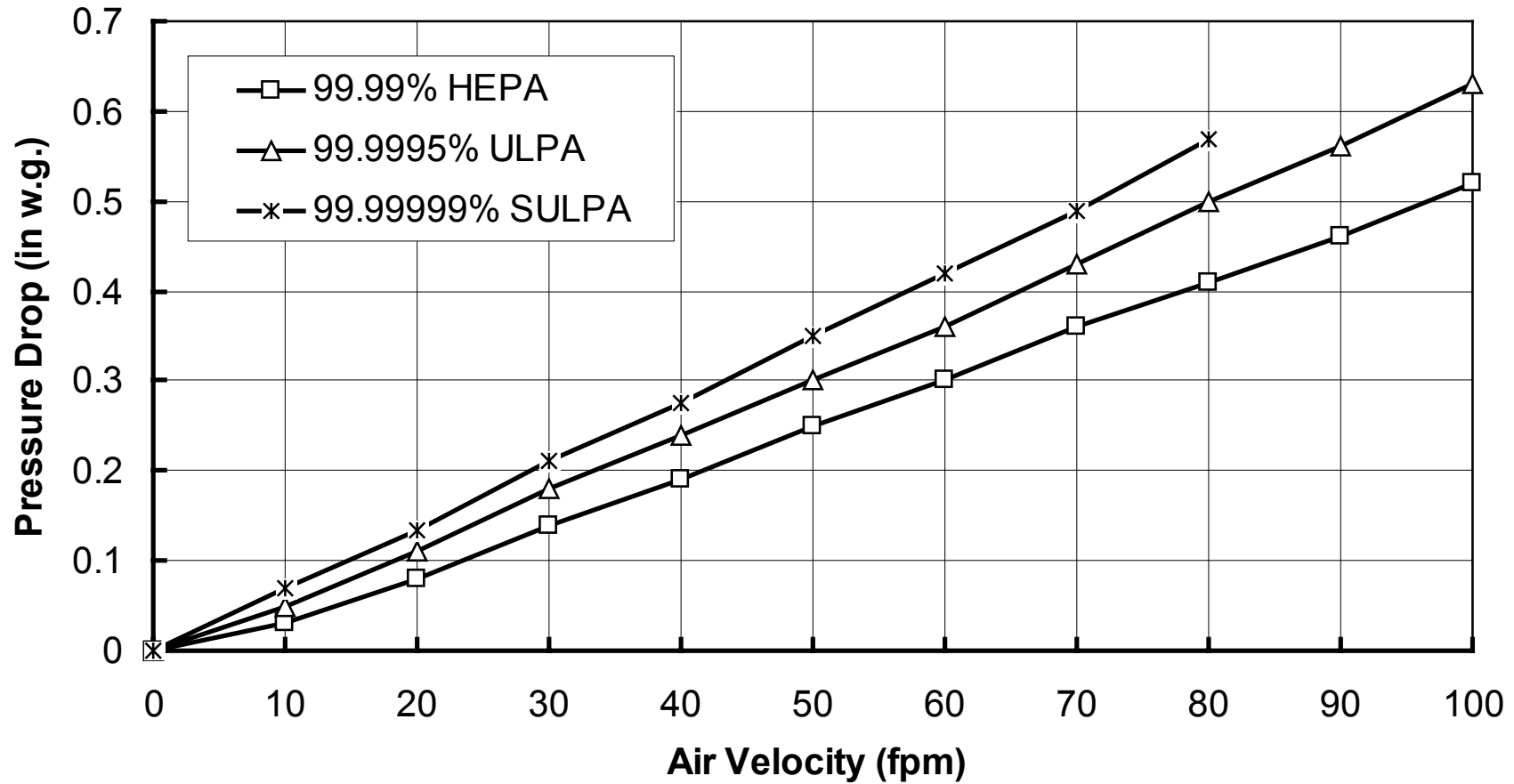
Dimple Pleat - 2" Pressure Plenum Filters Pressure Drop vs Velocity
